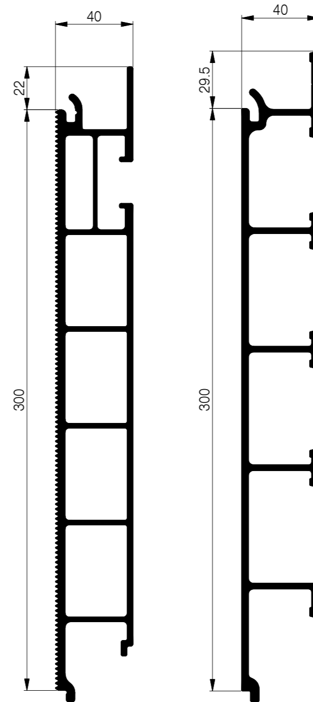
51 105 7.674 kg/m L = 7250 R
