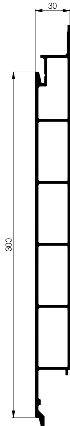
46 105 4.962 kg/m L = 6350 R
